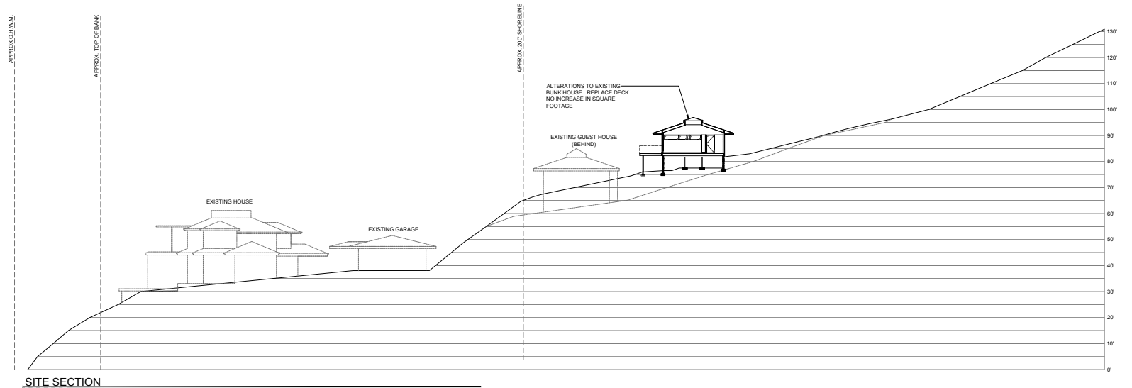
SITE SECTION
